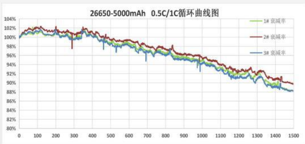
2.75V-4.2V 0.5C/1.0C Cycle @ RT
